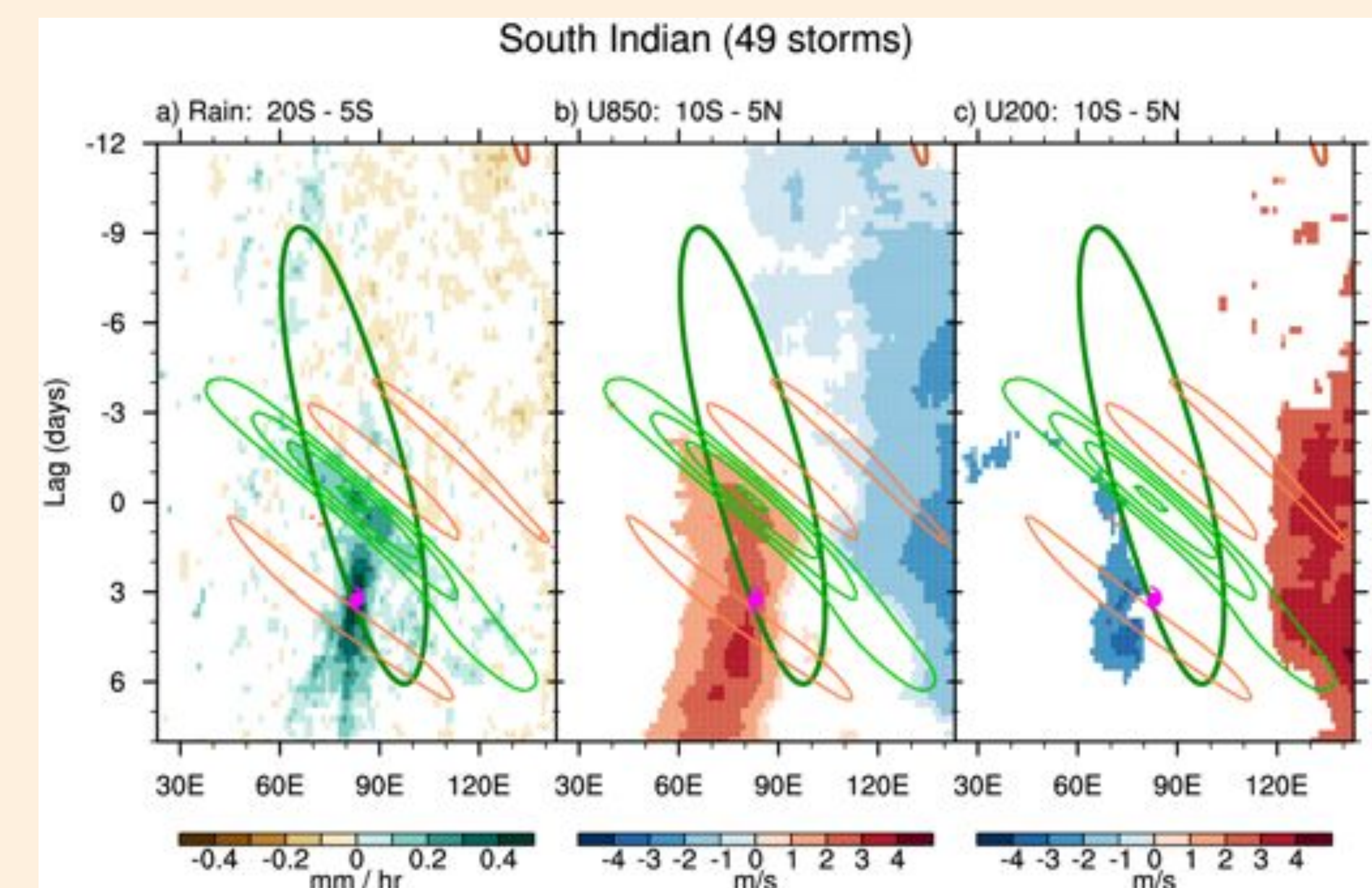
Composite TRMM rainfall for South Indian storms forming 3.00–3.75 days after Kelvin wave passage
