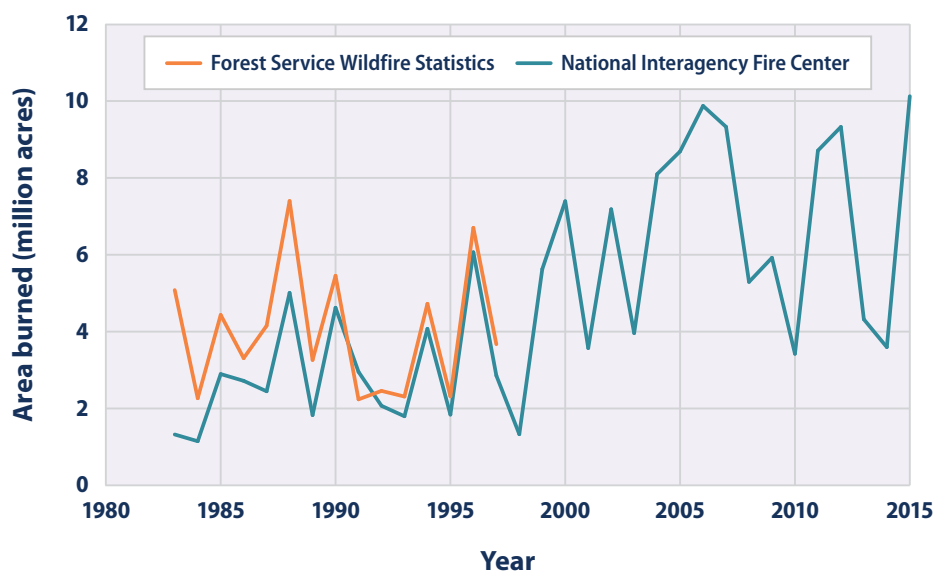
Wildfire Extent in the United States, 1983–2015
