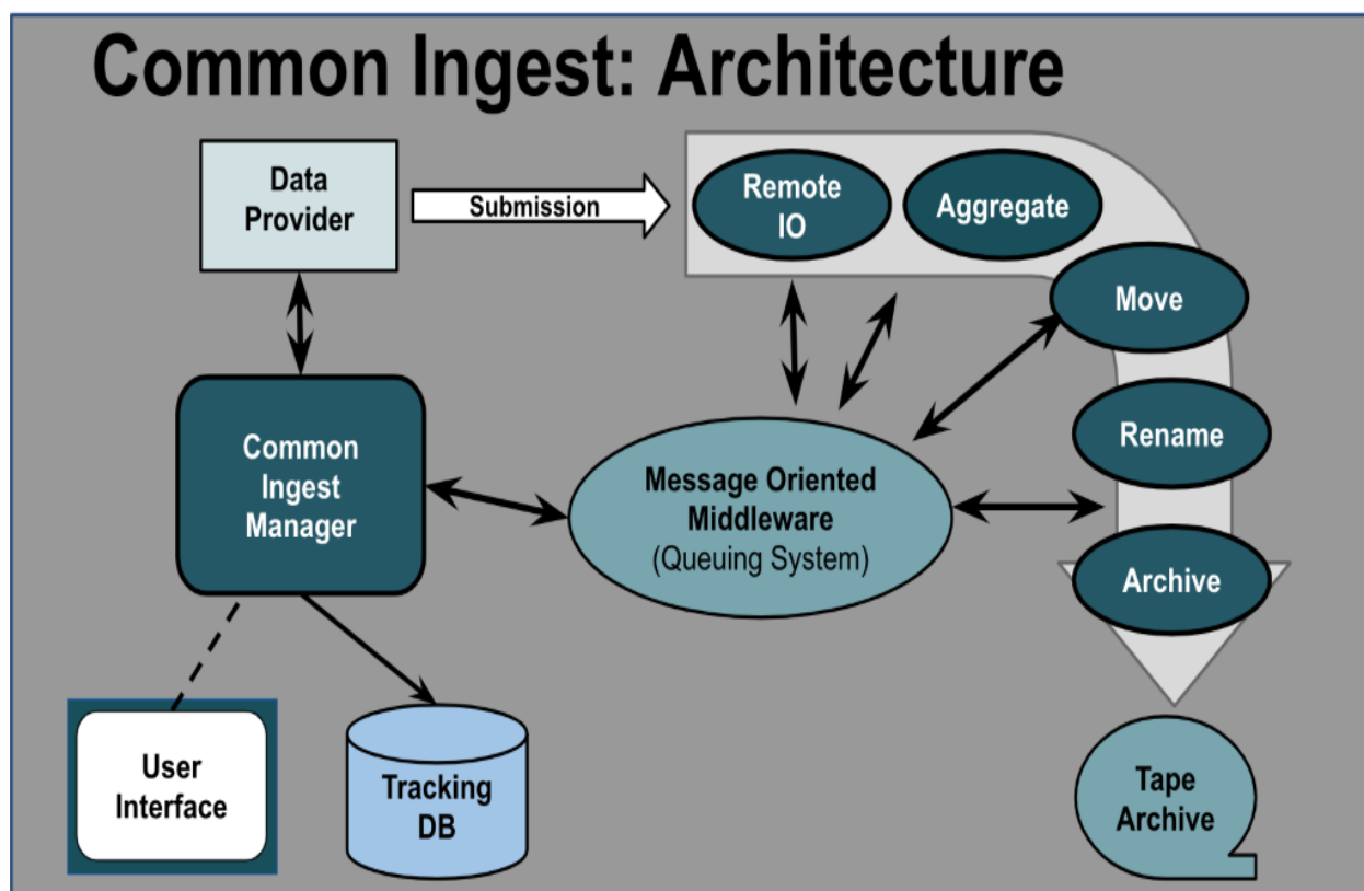
Figure 2. CI architecture.
