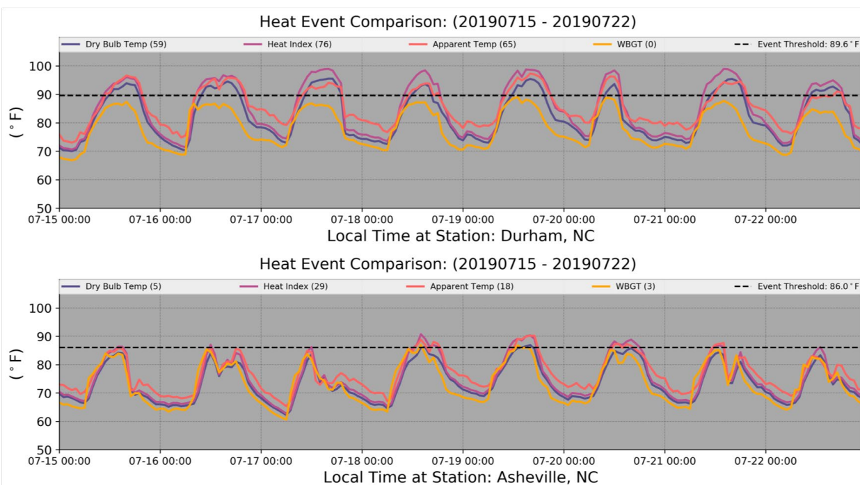
Figure 1. Time series of hourly heat indices for a heat event taking place between July 15th and July 22nd, 2019, in Durham, NC (top), and Asheville, NC (bottom). Number of hours above the heat event threshold are also displayed.
